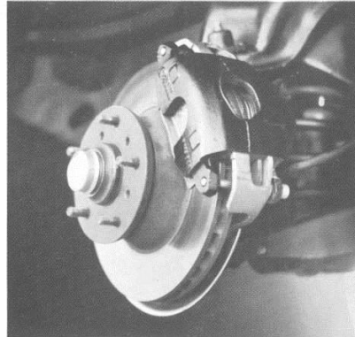
Power Disc Brakes, Front (Code 511—UPC JL2). New single-piston, floating-caliper design provides same braking area as 4-piston type. Power assist standard with disc brake. Available all models. (F)
