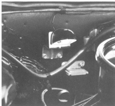
Underhood Lamp (Code 671—UPC U26). Available for all models, all series—included in Lamp Group (Code 322). Light floods entire engine compartment. Activated by the hood spring, it lights automatically when hood is raised. (F,D)
