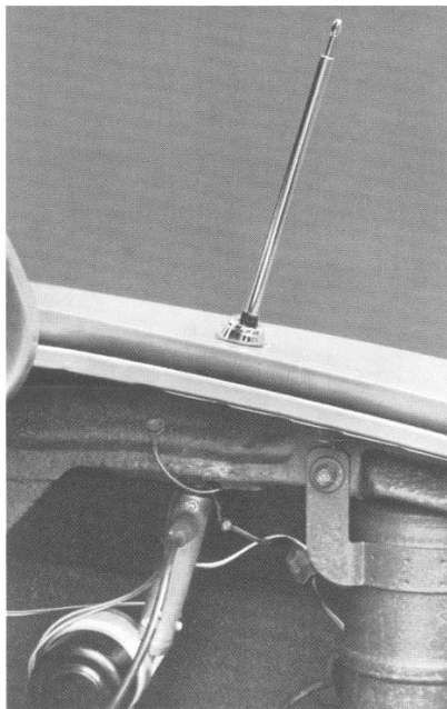
Electric Power Antenna (Code 381—UPC U75). Available with all radios on all models except Custom S Station Wagon, LeMans Safari and Grand Prix. Raises and lowers antenna by a switch on the instrument panel. Antenna is mounted on the right rear fender. (F)
