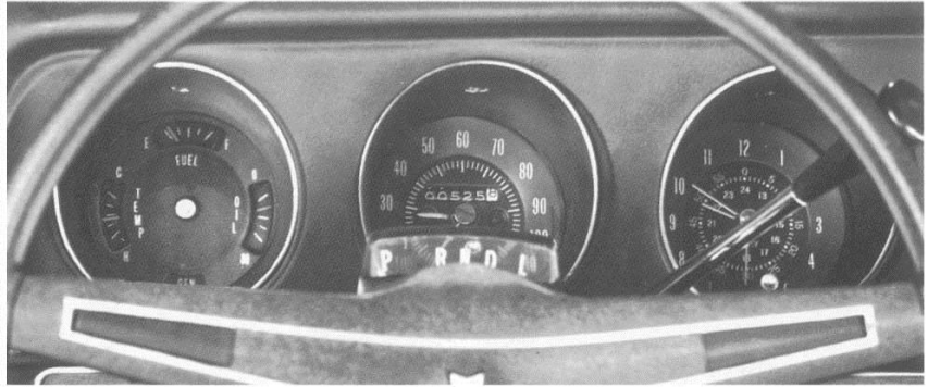
Rally Gauge Cluster & Rally Clock (Code 484—UPC W63). Integrates speedometer, oil-water-fuel-battery monitors and sweep second hand rally clock. Or rally clock can be replaced with Instrument Panel Tachometer
