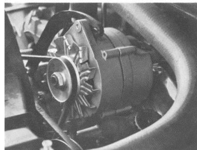
Delcotron Alternator-Regulator (62-Amp. Code 681—UPC K81; 55-Amp. Code 682—UPC K82; Self-regulated 55-Amp. Code 688—UPC K96). Special "solid state" voltage regulator, built into the alternator, provides improved voltage control and added reliability—increases battery life. Available for all series equipped with V-8 engines. Style and amperage determined by engine or equipment. (F)
