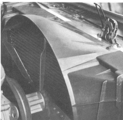
Heavy-duty Radiator (Code 701—UPC V01). Has greater cooling capacity; standard with air-conditioned cars. Available for all models. Also, SUPER-COOLING, HEAVY-DUTY RADIATOR (Code 702—UPC V02), for cooling under most severe driving conditions. Available for Catalina, Executive and Bonneville. (F)
