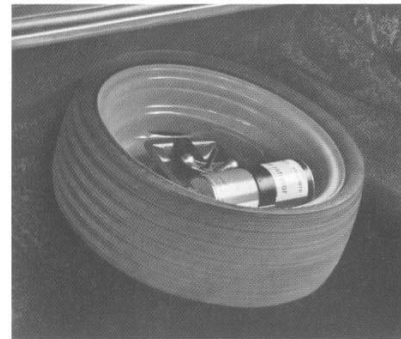
"Space-Saver Spare" Tire (Code 704—UPC N65). Available for all Tempest and Grand Prix models—standard on Firebird. Adds approximately 3 cubic feet of usable luggage capacity. Easily inflated with handy pressure can and provides many miles of spare tire driving. (F) New "Space-Saver Spare" Tire Inflators for replacement available from dealer. (D) Also, see "Instant-Aire" Pump—this page.
