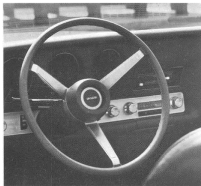
Custom Sports Steering Wheel (Code 462—UPC N34). One style available for all models. New shallow design and new molded vinyl hub with center horn button ornament. It has a smart, simulated wood appearance and three, equally spaced, bright steel spokes. (F)
