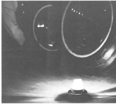
Underhood Utility Lamp (Code 671—UPC U26). Available for Catalina, Executive and Bonneville models—included in Lamp Group (Code 322). Ideal for emergencies after dark. Features 17 feet of self-storing extension cord. (F,D)
