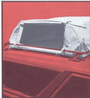
Luggage Carrier Cover . Water and dust-resistant fabric protects luggage. Side opening can be locked. Cover folds flat when not in use. Easily attached to luggage carrier. (D)
