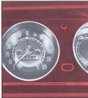
Safeguard Speedometer & Fuel Warning Lamp (Code 634) . Warns of excess speed and low fuel. Control knob lets you select desired speed limit. Buzzer and light signal you when car exceeds this speed. Another light tells you when to refuel. Not available with Rally Instrument Cluster. (F)
