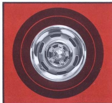
Rally Wheels (Code 691) . . . with special 7.75 x 14 tires only. Highly functional as well as extra sporty. Large openings provide maximum cooling for brakes. Includes stainless steel cap, chrome plated wheel nuts and stainless steel full trim ring. (F)
