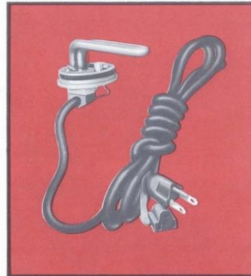
Engine Block Water Heater . Electric engine-coolant warm-up units are designed to provide fast starts and quick heater action in severe cold. Overnight, single unit raises engine coolant temperature from 0°F. to 50°F., dual unit to about 90°F. Plugs into cord from standard house outlet. (D)
