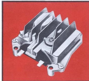
Full Transistor Voltage Regulator (Code 662) . Increases battery life, provides more accurate voltage regulation. No moving parts. No breaker points. Std. on V-8 engines with transistor ignition or Air Conditioning. (F)
