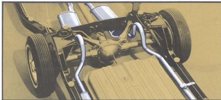
Dual Exhausts (Code 511) . . . cuts down back pressure in the exhaust system, adds to efficiency. Standard on Grand Prix and with 421 and 421 HO engine options, available on all other models. (F)
