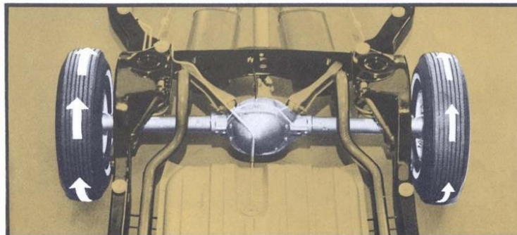
Safe-T-Track Differential (Code 701) . . . new design assures adequate pull when very low traction is encountered at one wheel. Also provides smoother transfer of torque from one rear wheel to another. (F)
