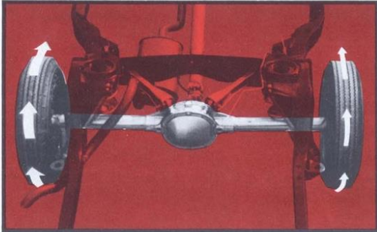
Safe-T-Track Differential (Code 701) . . . design assures necessary amount of pull when very low traction conditions are encountered at one wheel. Also provides smooth transfer of torque from one rear wheel to another. (F)
