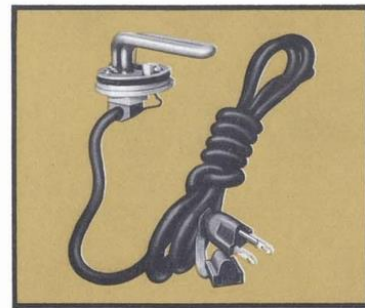
Engine Block Water Heater. Electric pre-heater for engine coolant helps provide fast starts, quick heater action in severe cold. Overnight, single unit raises engine coolant from 0°F. to 50°F., dual unit to about 90°F. Plugs into cord from standard house outlet. (D)
