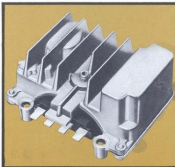
Full Transistor Voltage Regulator (Code 662) . Increases life of battery, provides better voltage regulation. No moving parts. No breaker points. Standard on all models with transistor ignition or heavy-duty 62 amp. alternator or air conditioning. (F)
