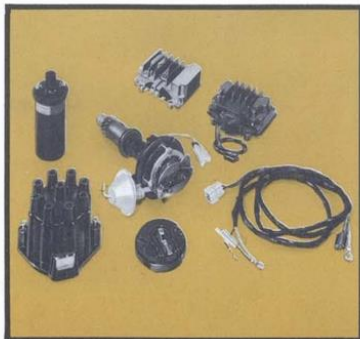
Full Transistor Ignition System (Code 671) . For all premium-fuel engines, all series. Provides ignition without condenser or mechanical contacts. Combines increased electrical output at high speeds with greater ignition stability and longer spark plug life. (F)
