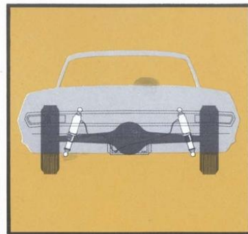
Superlift Shock Absorbers (Code 622). Help maintain level ride when trunk or trailer-tongue loads are extra heavy. Adjustable air spring is built into rear shock absorber. Tire-type air-filler valve. (F,D)
