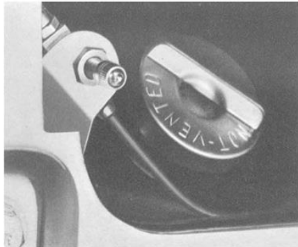
Superlift Shock Absorbers (Code 634). Available all models except Firebirds. Help maintain a level ride when trunk or trailer tongue loads are extra heavy. Adjustable air spring is built into rear shock absorber. Equipped with tire-type air filler valve for simple air fill at filling stations. (F, D)
