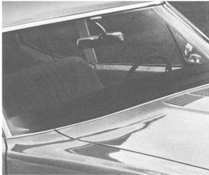
Concealed Windshield Wiper Linkage (Code 411). Available on all Tempest, Tempest Custom only. Standard on Le Mans, Tempest Safari and GTO. Part of Decor Group for these models. A dual-speed, fully concealed, tandem wiper with washer assembly featuring an articulating left wiper. Articulation feature on left arm wipes greater area for increased driver visibility. (F)
