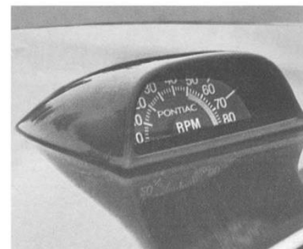
Tachometer (Code 434). New Pontiac design. Hood-mounted unit, installed outside the car in front of the windshield, in line with the driver's vision. Offers easy, instant reading. Available all models. (F, D)
