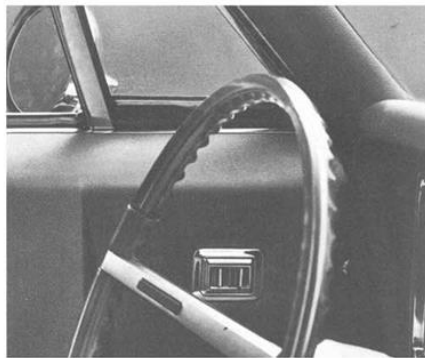
Power Vent Windows (Code 552). Operates vent windows by selecting the respective switch on the driver's side or activating the switch under the right vent window. Available along with power windows on Catalina, Executive and Bonneville models only. (F)
