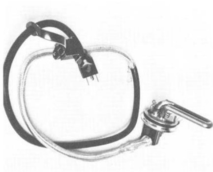
Engine Block Water Heater. Electric preheater for engine coolant provides fast, effortless starts, quick heater action during severe cold. Single unit raises engine coolant overnight from 0°F to 50°F, dual unit to about 90°F. Operates from standard house electrical outlet. (D)
