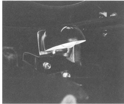
Underhood Lamp (Code 671). Lights automatically when hood is raised. Available and is part of Lamp Group—Code 332—for all models except Catalina, Executive, Bonneville and Grand Prix—where it is standard equipment. (F, D)
