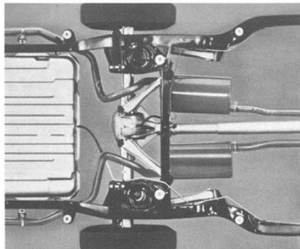
Dual Exhausts (Code 481). Cuts down back pressure in exhaust system, adds to engine efficiency. Available on all models with V-8 engines except station wagons. (Standard on Firebird H.O. Firebird 400, GTO and Grand Prix and all models equipped with H.O. V-8 engines.) (F)
