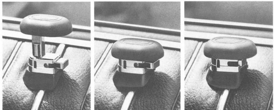
Rear-door Child Lock Guards (4-Door Models Only). Prevents children from unlocking and opening rear doors. When buttons are down and Lock Guards are pushed in, rear doors can't be opened without inserting key into lock button. 1—Unlock position. 2—Regular locked position. 3—Lock Guard position. Any of your regular car keys may be used to release the Lock Guards. (D)
