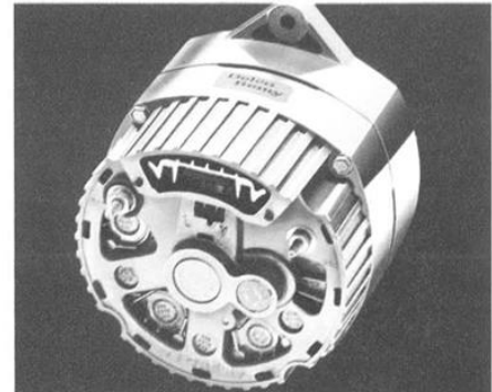
Delcotron Alternator-regulator (Code 694—42 AMP.) (Code 698—55 AMP.) This new and unique "solid state" voltage regulator provides improved voltage control and added reliability —increases battery life. Available for Catalina, Executive, Bonneville models. Standard on Grand Prix. (F)
