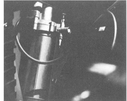
Automatic Level Control. Available only with Superlift Shock Absorbers. A vacuum-operated air compressor, mounted in the engine compartment, automatically keeps the rear of the car at a constant height when fully loaded. Available Catalina, Executive, Bonneville and Grand Prix models only. (D)
