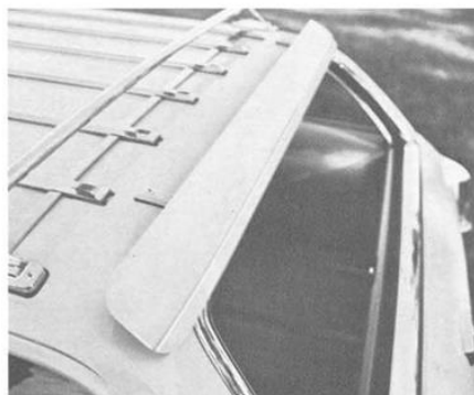
Station Wagon Rear-window Deflector (Code 408). Horizontal metal vane directs air stream down onto rear window to help keep it free of dust. Also promotes quieter ventilation of interior when cowl vents are opened, side windows closed and rear window open. Available for all station wagons. (F, D)
